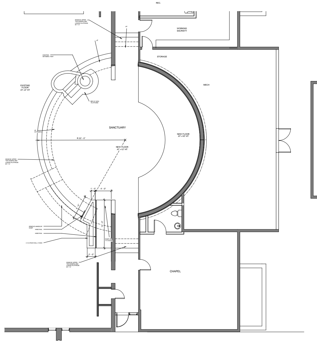
1 Floor Plan Sanctuary 1/4" = 1'-0"
